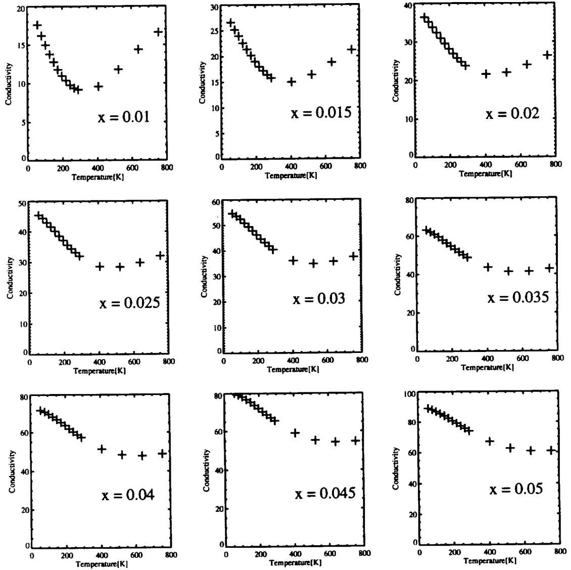
Figure 3.1a Conductivity as a function of temperature for r=1.0 .
